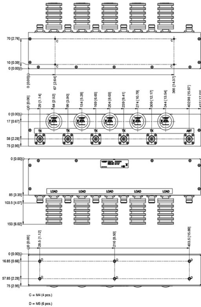
MOUNTING DETAILS
