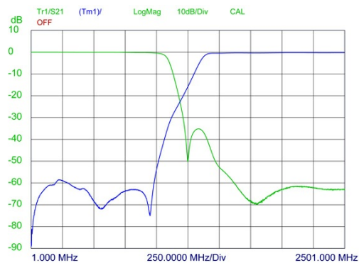
TYPICAL RESPONSE CURVES - 1 DB
