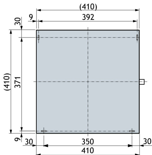
MOUNTING DETAILS (DIMENSIONS EXCL. COVER)
