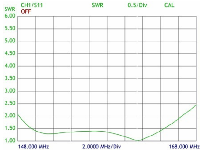
TYPICAL GAIN AND VSWR CURVE
