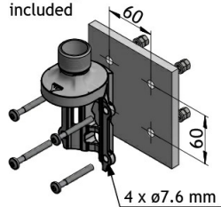
Bolts for wall mounting not included
