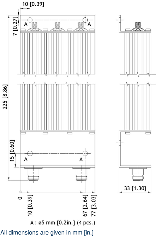
MOUNTING DETAILS
