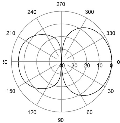
E-Plane | 405 MHz
