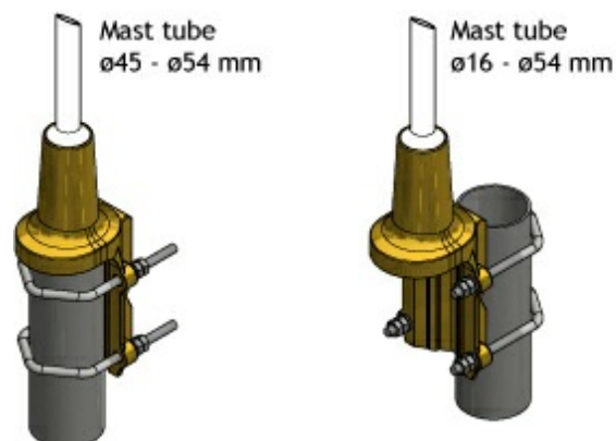
MULTI-PURPOSE MOUNTING BRACKET
